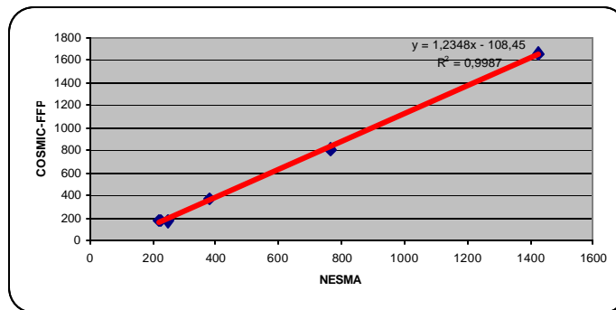
Figure 3c Vogelezang & Leterthuis data graph (more than 200 NESMA points)
