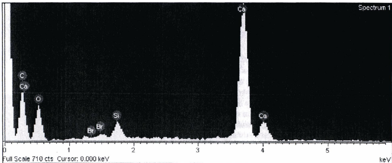
Figure 3 b: Element analysis at detail shown in Fig. 3 a
