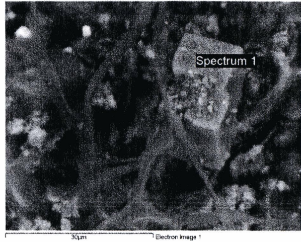
Figure 3 a: Copán stone flake with calcite and fungi on flake surface, ESEM/EDS.
