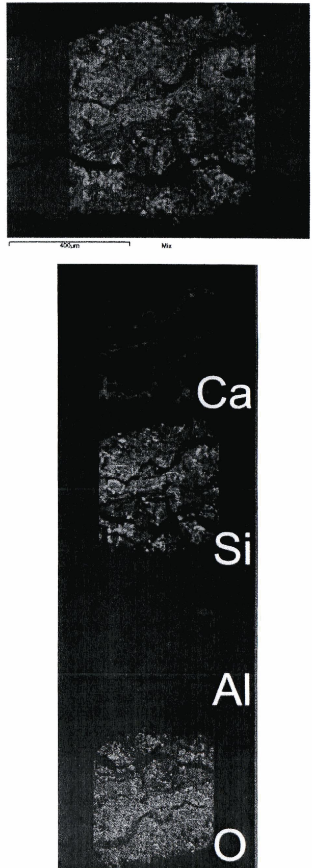
Figure 2: ESEM/EDS image of Copán stone flake in BSE mode with X-ray overlay showing distribution of calcite in fractures (false color-red). Scale is 400 microns.
