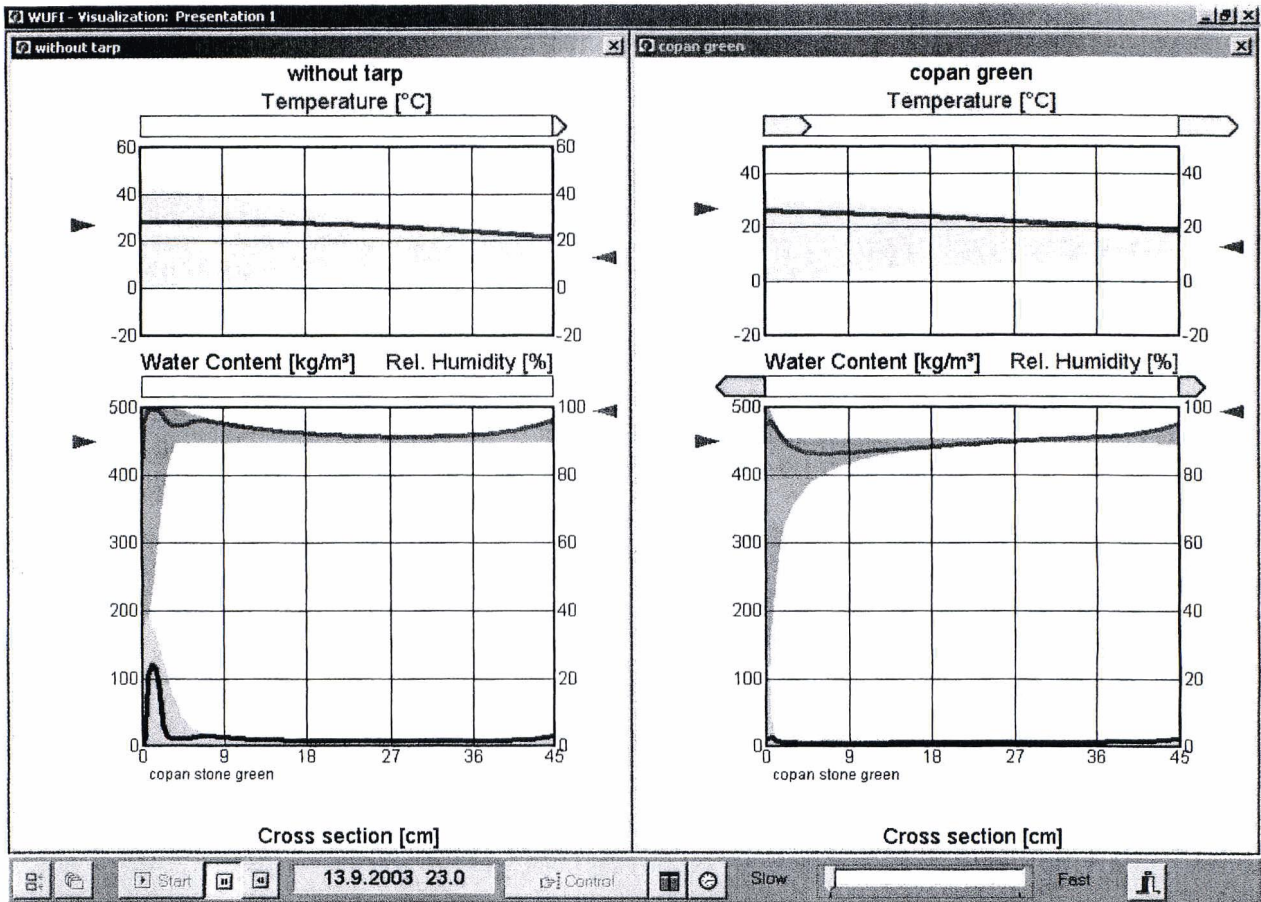
Figure 5: WUFI-Calculation for depth profiles of water content, relative humidity and temperature for the Copán staircase (green stone) with (right) and without (left) the tarp.
