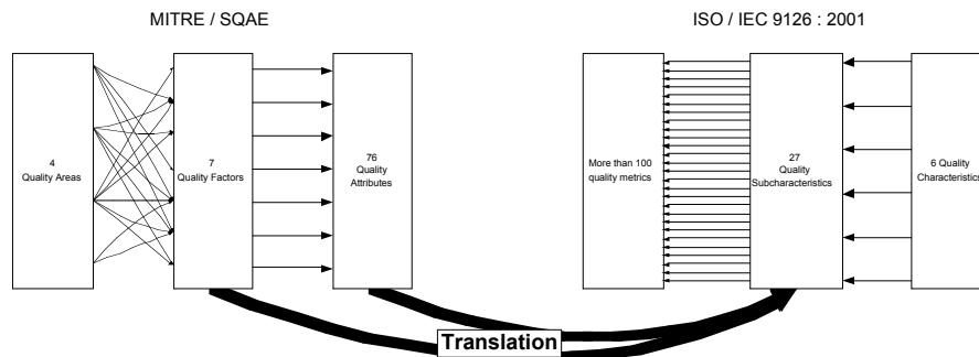
Figure 8: The translation activity
