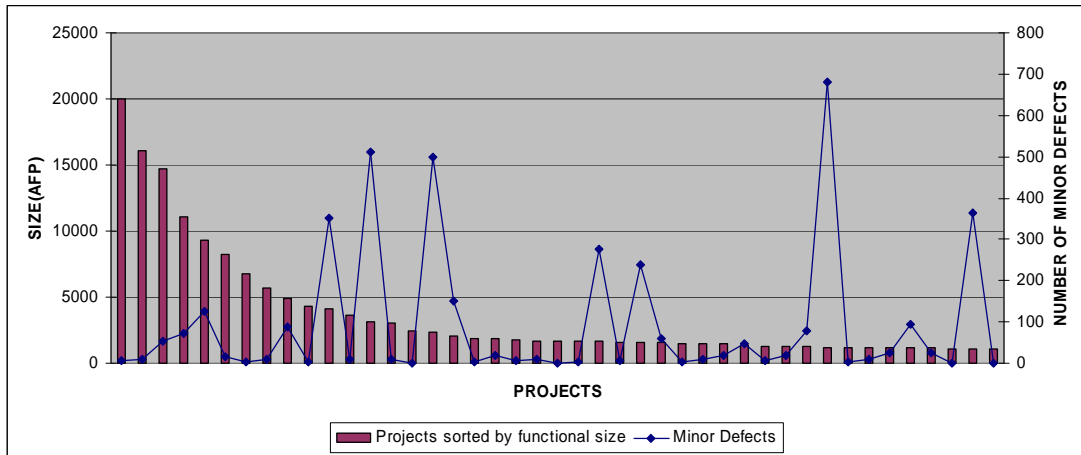
Figure IV.7 Number of Minor Defects and Size per Project (43 projects).
