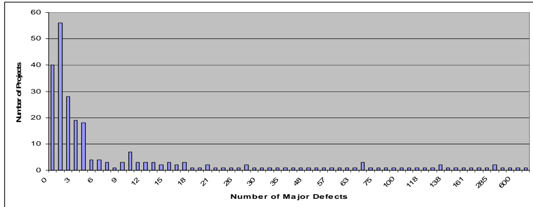
Figure IV.2 Project classification by Number of Major Defects (252 projects).
