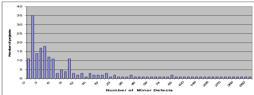
Figure IV.1 Project classification by Number of Minor Defects (200 projects).
