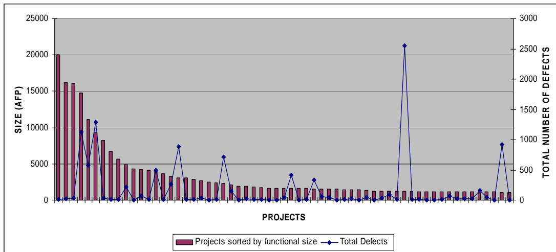
Figure IV.10 Total Number of Defects and Size per Project (61 projects).
