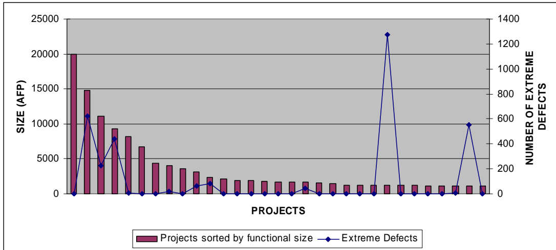
Figure IV.9 Number of Extreme Defects and Size per Project (31 projects).
