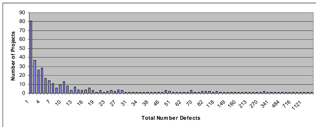
Figure IV.4 Project classification by Total Number of Defects (361 projects).
