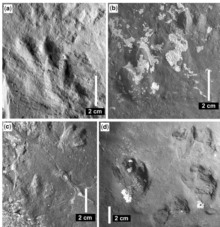
Fig. 7. Pes and manus imprints of cf. Brachychirotherium : (a) plaster replica taken from slab MGUH 31233a with two overprinted pes impressions; (b) & (c) natural casts from slab MGUH 31235; and (d) natural mould from a different slab (MGUH 31234).
