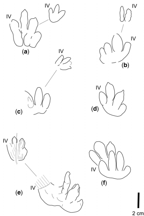
Fig. 10. (a)–(f) Sketches of footprints of cf. Brachychirotherium from the Ørsted Dal Member. The outlines refer to specimens in the following figures: (a) Figure 4b–c; (b) Figure 5b; (c) Figure 7c; (d) Figure 5c; (e) Figure 6b; and (f) Figure 7a. Their position on the slabs is indicated by corresponding letters in Figures 8 and 9. Note tetradactyl preservation and lack of digit V.
