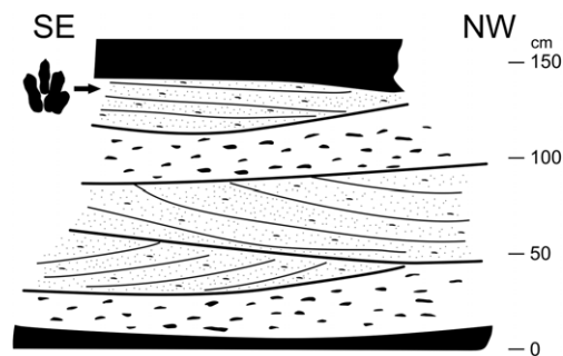
Fig. 3. Sketch of sedimentology at the Lepidopteriselv footprint locality with the position of the track level.
