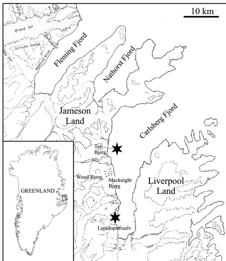
Fig. 1. Map showing the study area and the position of the footprint localities.
