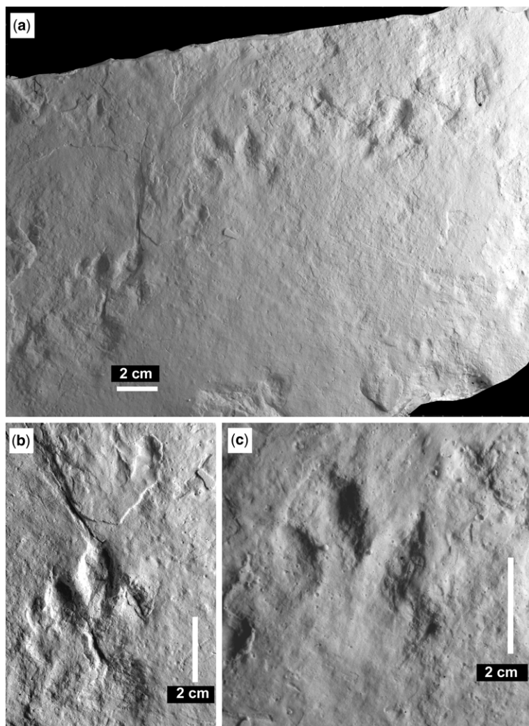
Fig. 5. Plaster replica of the lower portion of the slab in Figure 4 (MGUH 31233a). (a) Several pes and manus imprints; (b) & (c) detail of (a).
