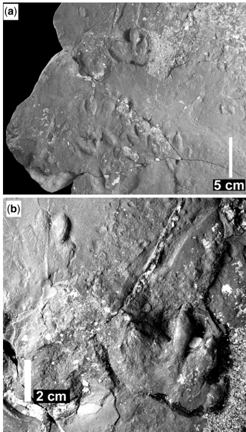
Fig. 6. Slab MGUH 31235 with several pes and manus imprints of cf. Brachychirotherium preserved as natural casts (convex hyporeliefs): (a) overview of the larger section; and (b) detail with a possible pes–manus set. Note dragmarks of scales in the manus.
