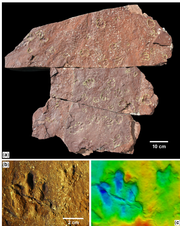
Fig. 4. Archosaur footprints cf. Brachychirotherium from the Ørsted Dal Member of the Fleming Fjord Formation (Upper Triassic, Norian–Rhaetian) of eastern Greenland. (a) Overview of slab MGUH 31233a–c (broken into three pieces: 31233a is the lower, 31233b the middle and 31233c the upper part) with numerous small pes and manus imprints of cf. Brachychirotherium preserved as concave epireliefs and outlined with chalk. (b) & (c) Detail of a pes–manus set from the middle part of the slab (MGUH 31233b): (b) photograph of natural mould and (c) a 3D model.
