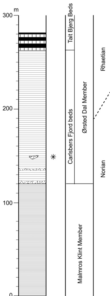
Fig. 2. Stratigraphic section of the Triassic of Greenland with the position of footprints described here marked with an asterisk. Stratigraphic section based on observations at Lepidopteriselv. The boundary between the Norian and the Rhaetian was placed at about 208.5 Ma in the middle of the Carlsberg Fjord beds in a nearby section by Clemmensen et al. (1998). New evidence from high-precision U–Pb geochronology, however, places this boundary at about 205.5 Ma (Wotzlaw et al. 2014), suggesting that the Norian–Rhaetian boundary should be moved upwards in the East Greenland section.
