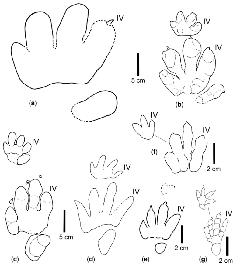
Fig. 11. (a)–(e) Sketches of Brachychirotherium pes and manus from different Upper Triassic localities. (a) Brachychirotherium hassfurtense (type ichnospecies, lectotype) from the Hassberge Formation (Late Carnian, Upper Triassic) of northern Bavaria, Germany. (b) B. thuringiacum from same stratum and locality as (a). (c) B. parvum (holotype) from the Passaic Formation (Norian, Upper Triassic) of New Jersey, USA. (d) B. parvum from the Redonda Formation (Norian–Rhaetian, Upper Triassic) of New Mexico, USA. (e) B. isp. from the Los Colorados Formation of NW Argentina. (f) cf. Brachychirotherium from the Ørsted Dal Member of the Fleming Fjord Formation (Upper Triassic, Norian–Rhaetian) of eastern Greenland. (g) Batrachopus from the Newark Supergroup (Lower Jurassic) of North America. From Klein & Lucas (2010a, b).
