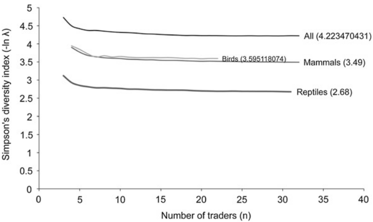
Fig. 19.6 Cumulative diversity curve for the Simpson's diversity index ( -\ln \lambda )
