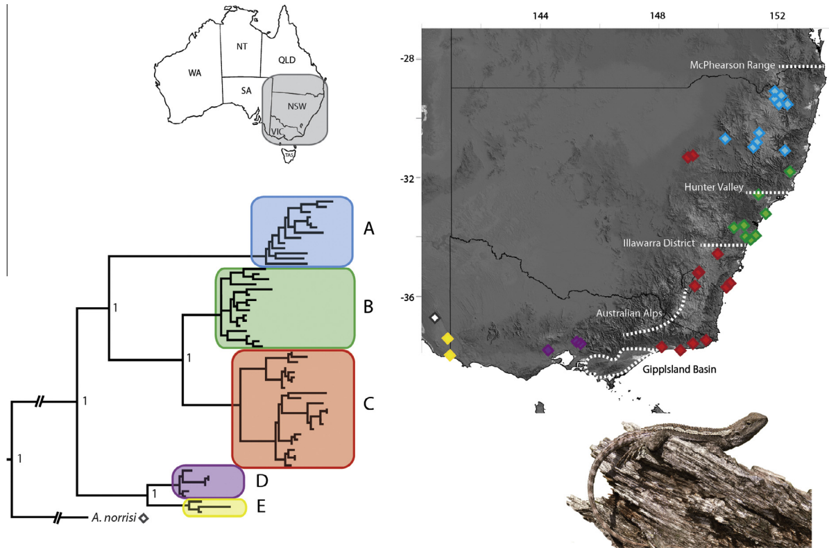
Fig. 1. Phylogeny of 62 Amphibolurus muricatus samples and outgroups based on the combined nd2 , nd4 , rag1 , bdnf and prlr data, and their distribution across eastern Australia. Here we show the relationships among the five clades (A–E) based on the *BEAST species-tree analysis. Numbers beside nodes refer to posterior probabilities. Dark lines on the map represent State boundaries. WA = Western Australia, NT = Northern Territory, QLD = Queensland, SA = South Australia, NSW = New South Wales, ACT = Australian Capital Territory, TAS = Tasmania. White stippled lines indicate biogeographic barriers mentioned in the text. Colored diamonds indicate our sampling for each A. muricatus clade, with the white diamond representing our sample of A. norrisi . For the Maximum likelihood phylogeny showing individual details of each A. muricatus sample see Appendix Fig. 2 . Photo: Ben Twist.
