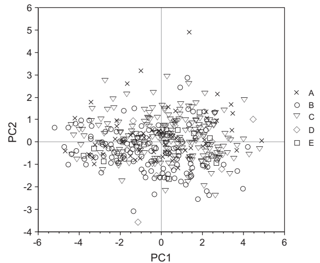
Fig. 2. Summary of results for the PCAs of the morphological data for 437 A. muricatus specimens which we assigned to 5 clades (A–E) based on genetic and geographic data.
