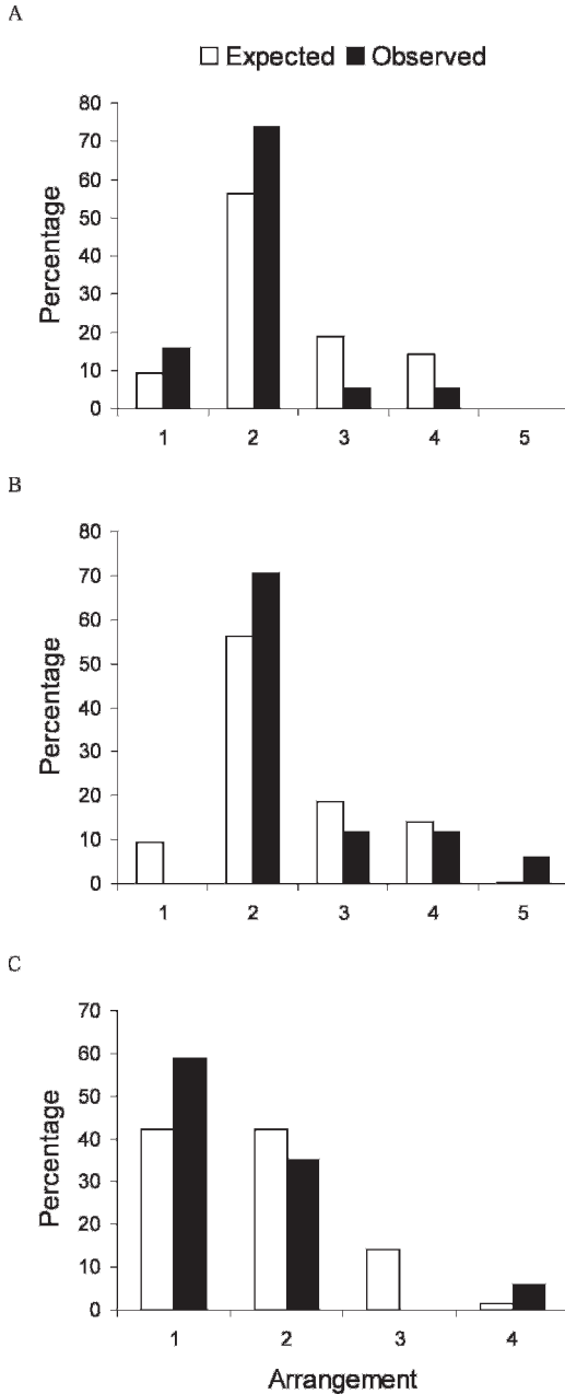
FIG. 1. The observed and expected spatial arrangement of Platysaurus broadleyi in selected grouping experiments in which the number of available refugia equalled the number of lizards. (A) Four males; (B) one male and three females; and (C) one male and three females in which the possible spatial distribution is in relation to the male (i.e., male and one female together under same tile, male and two females under same tile, etc.). Males avoided grouping with other males significantly more than expected by chance, whereas male:female grouping was not significantly different from chance (see text for statistical analysis). For (A) and (B) the x-axis numbers correspond to the
