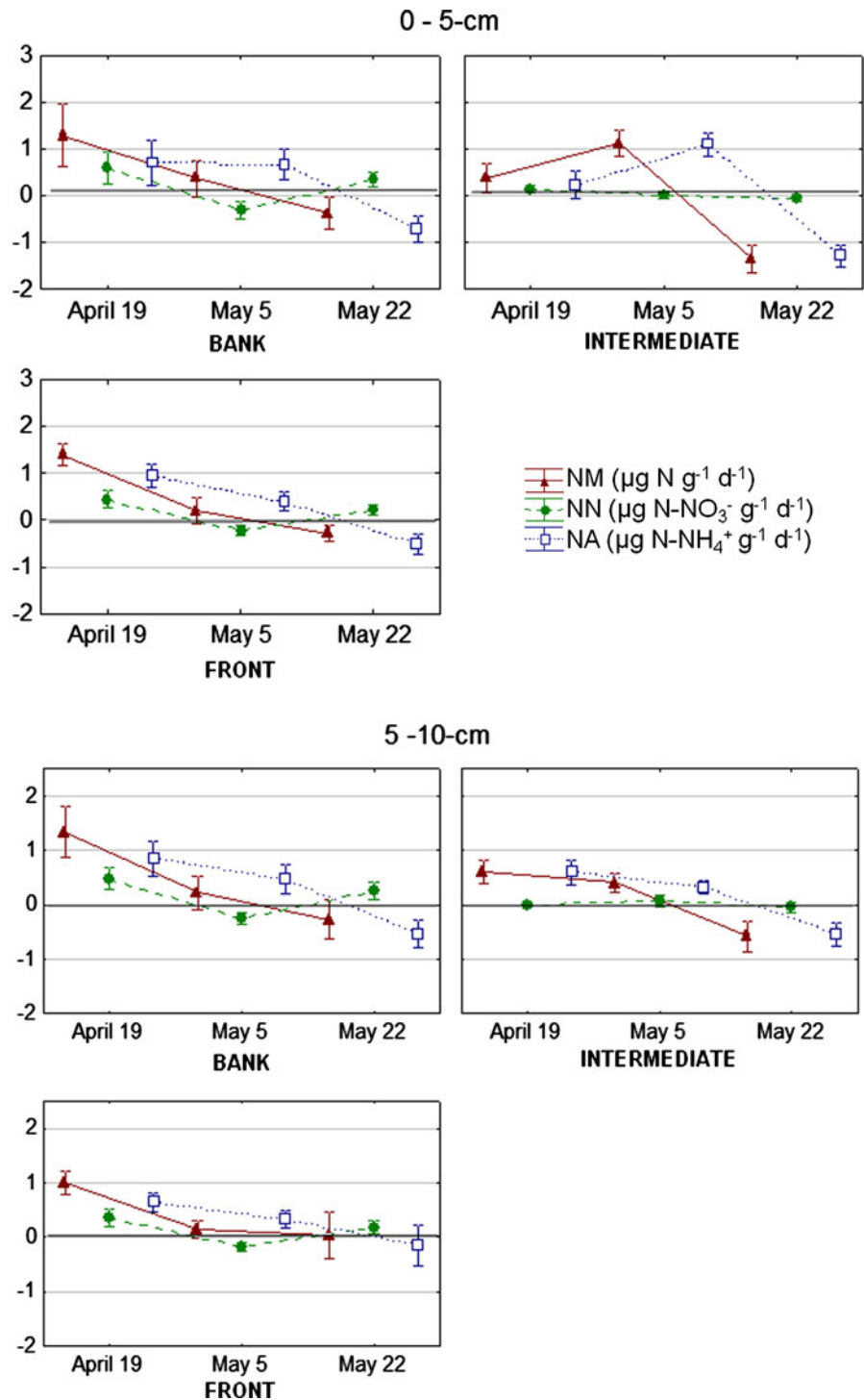
Fig. 6 Evolution of soil net N mineralization (NM), nitrification (NN) and ammonification (NA) rates (mean \pm SE; n = 9 ) during the experiment for the each station and at two soil depths (0- to 5-cm, 5- to 10-cm). Values given for T1 (April 19th), T2 (May 5th) and T3 (May 22nd) integrate the elapsed time between that sampling day ( T_n ) and the previous sampling day ( T_{n-1} ); see the “Materials and methods” section for details
