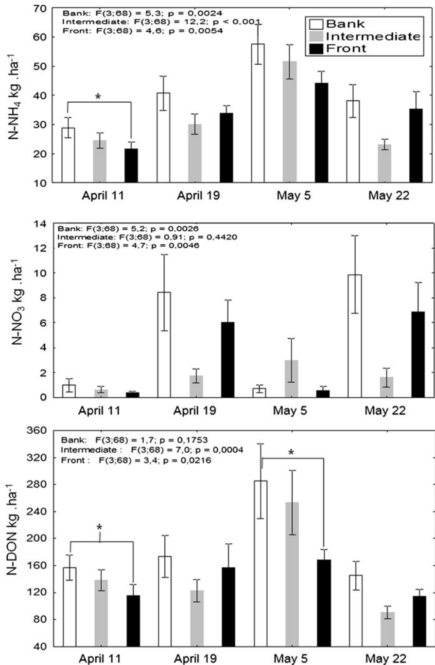
Fig. 4 Soil-N-NH 4 + , N-NO 3 - , and dissolved organic-N contents (mean ± SE, n = 18) for each station and the four sampling times: April 11th (T0), April 19th (T1), May 05th (T2), and May 22nd (T3). The data from the two depths were pooled by station. Intersampling time differences (significant at p < 0.05) for each N forms and station were tested and results ( F and p values) are inserted in each graph. Asterisks above bars give p levels of inter-station differences based on a Mann-Whitney test (* p < 0.05)
