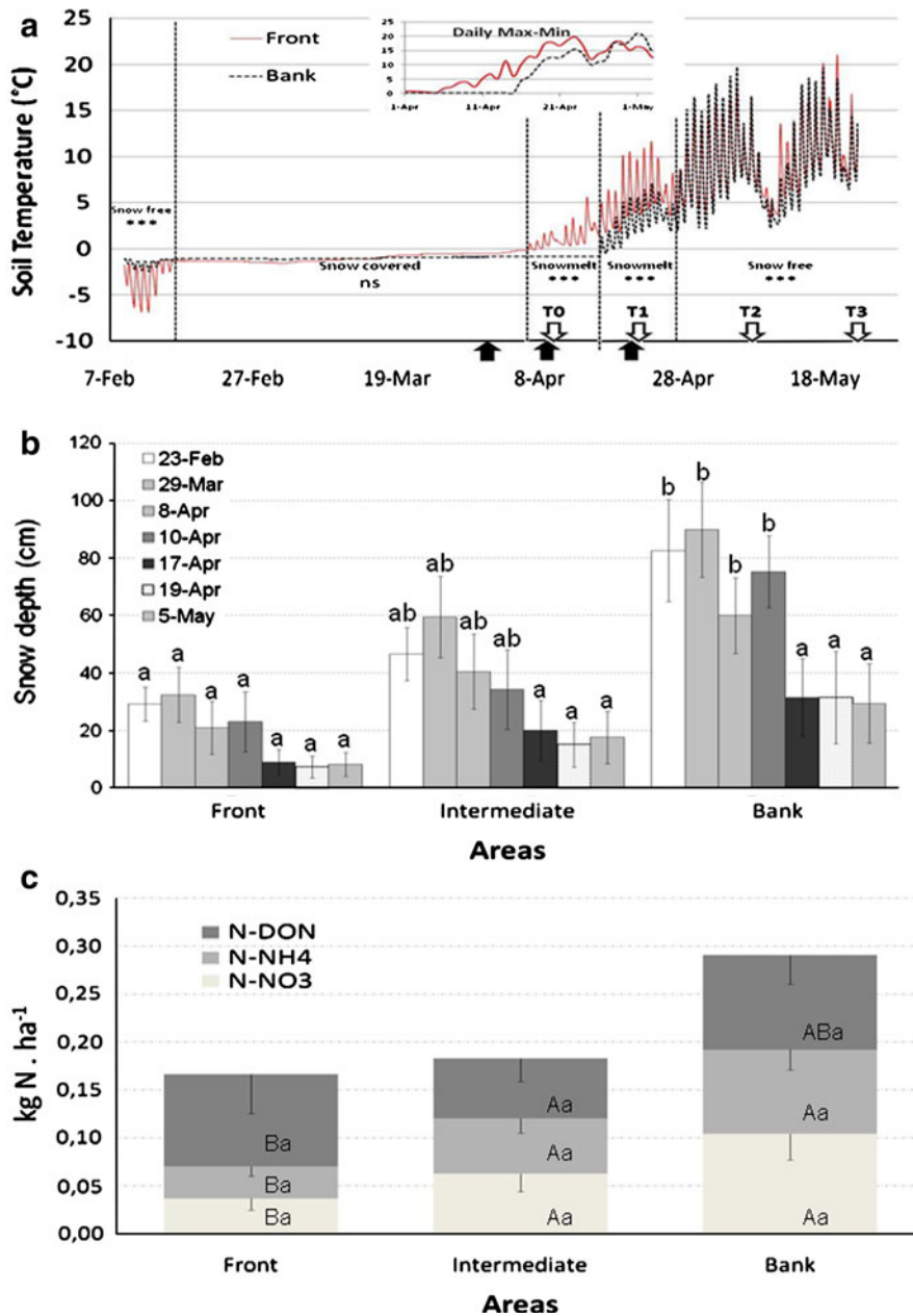
Fig. 2 a Time sequence of hourly mean soil temperatures at the front and the bank stations averaged from the triplicated subalpine terraces. White arrows represent soil samplings: April 11th (T0), April 19th (T1), May 05th (T2), and May 22nd (T3). Black arrows represent snow samplings (March 29th, April 8th and 17th). Dashed lines delimit time periods used for Wilcoxon non-parametric t tests: *** p < 0.001 ; NS not significant). The insert graph shows averaged daily differences between maximum and minimum temperatures for each station during the snow melt period. b Time sequence of snow depths (mean \pm SE, n = 9 ) measured on seven occasions between February and April for each station. Differences in snow depth
