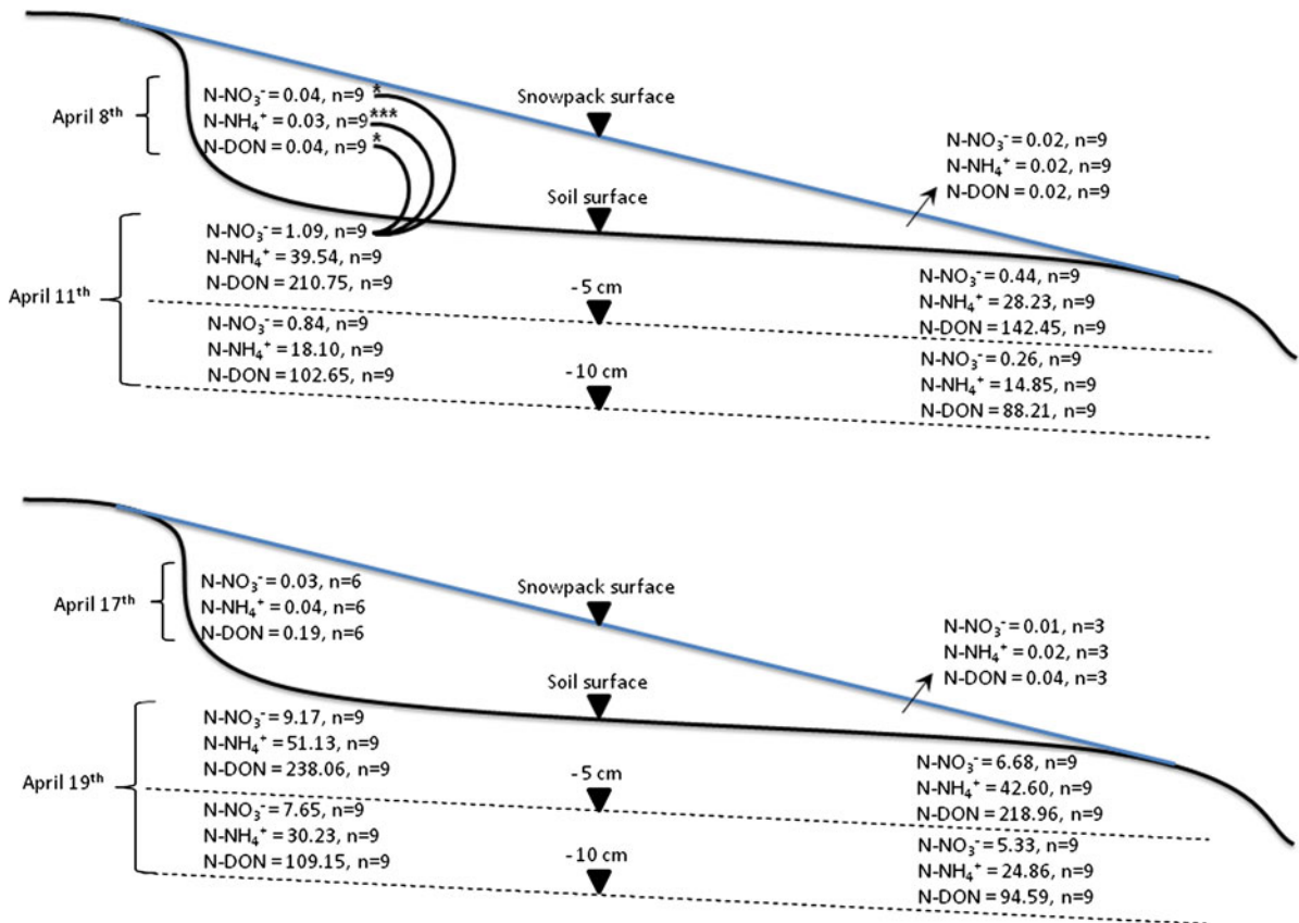
Fig. 5 Mean N stocks ( \text{kg}\cdot\text{ha}^{-1} , n = 9 , standard errors are not reported) measured simultaneously in the snowpack and the soil layers along the terrace toposequence (bank and front stations) at two different times during snowmelt. N is variable for snow data depending on the actual presence of snow. When
