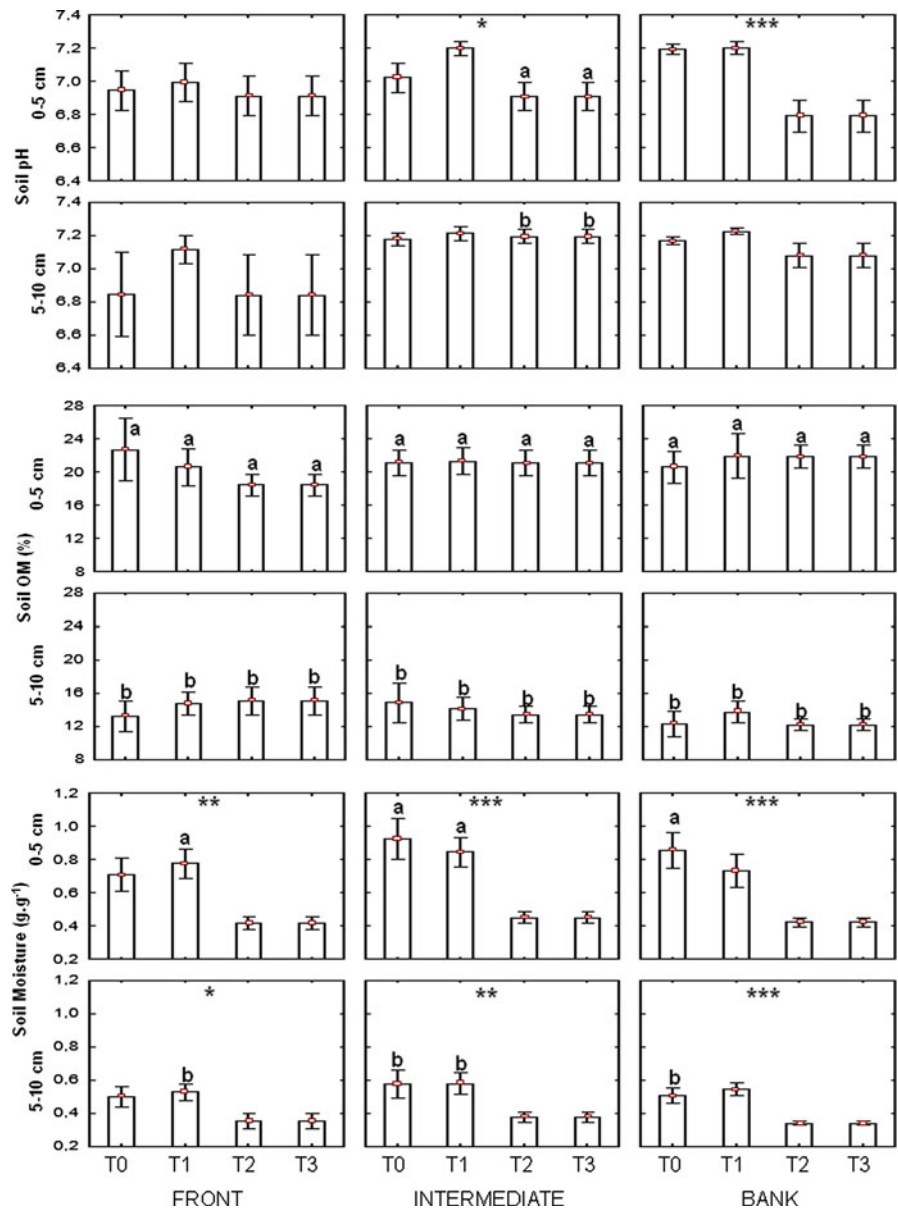
Fig. 3 Mean values ( n = 9 ; \pm SE) of soil pH, soil organic matter content and soil moisture at two depths (0- to 5-cm, 5- to 10-cm) and four sampling times: April 11th (T0), April 19th (T1), May 05th (T2), and May 22nd (T3). Different letters above the bars show significant differences ( p < 0.05 ) between depths using a Mann–Whitney U test. Asterisks above graph show the significance of inter sampling time differences using a Kruskal–Wallis Test (** p < 0.001 ; * p < 0.01 ; * p < 0.05 )
