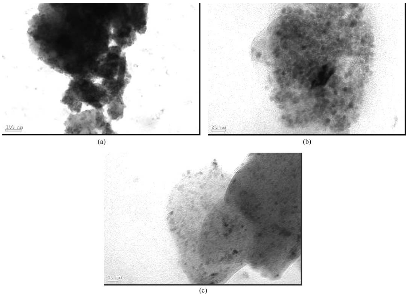
FIG. 4. TEM images for different mass loadings of mesostructured kaolinite substrate (a) 5% (w/v), (b) 10% (w/v), (c) 15% (w/v).
