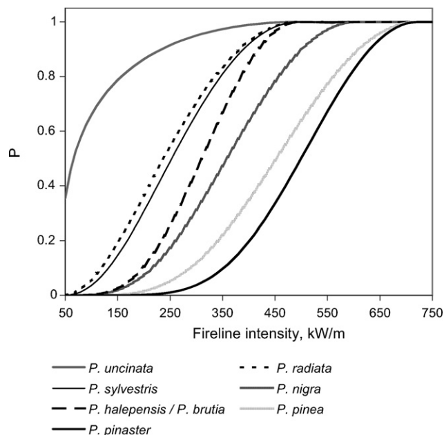
Fig. 2. Probability of post-fire tree mortality for different European pines calculated as per Peterson and Ryan (1986) for a range of hypothetical fireline intensities. A 8-m tall tree, with a crown length of 6.5 m and a diameter of 15 cm was assumed.
