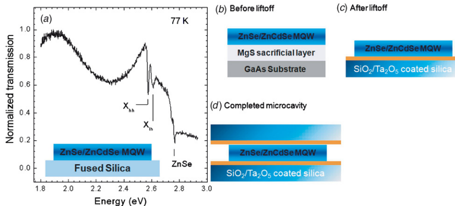
Figure 1. (a) Normalized transmission of the ZnSe/ \text{Zn}_{0.9}\text{Cd}_{0.1}\text{Se} QWs used as the active medium of the MC. Reference samples were lifted and transferred to a fused silica substrate. Inset: schematic of the QWs transferred to a glass substrate. (b)–(d) Schematics of the sample at each stage of the MC fabrication (not to scale).
