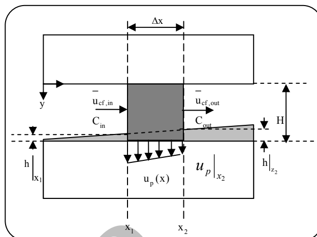
Fig. 3: Element used for mass balance.
