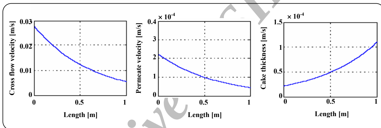
Fig. 4: Profiles in steady condition [10], [11].
