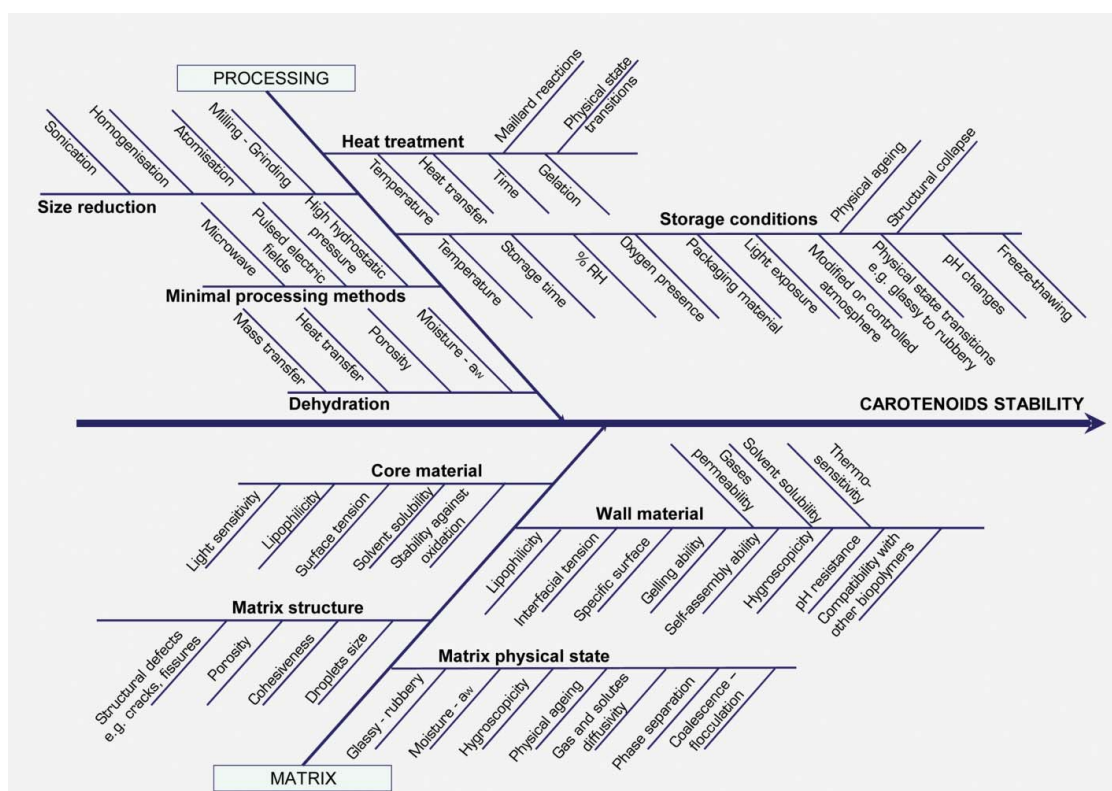
Figure 1. Cause and effect diagram illustrating parameters associated with processing conditions and matrix compositional and structural characteristics influencing the chemical stability of carotenoids.
