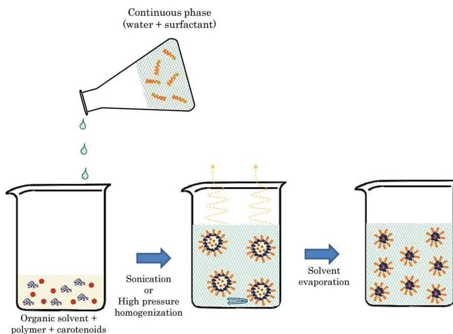
Figure 7. Illustration of the production of encapsulated carotenoids into nanoparticles using the emulsification—solvent evaporation method.
